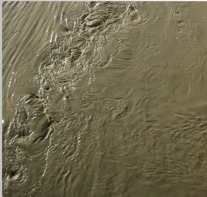
Figure 1: An everyday example of a shear flow, the Arno showing the generation of vortices in the boundary layer with the walled side of the river (right) and a freely flowing shear (left). The mixing and turbulent eddies are examples of what would be expected in the interaction regions in the inner disk.
